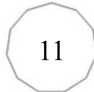
hendecagon
