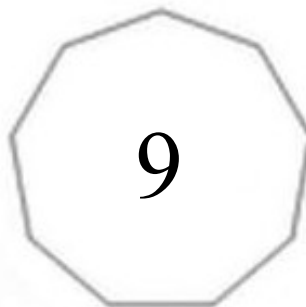
nonagon
