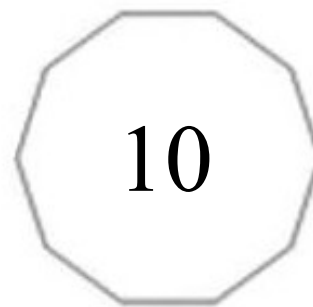
decagon
