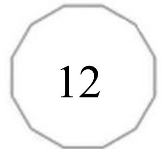
dodecagon
