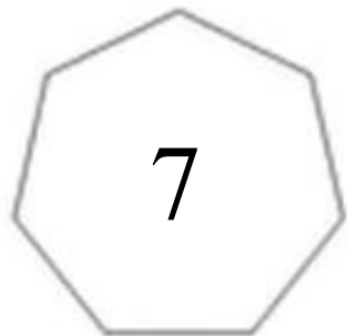
heptagon
